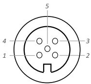
M12 5-Pin Connector A-Coding Male
